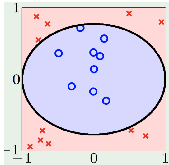
Nonlinear Model
